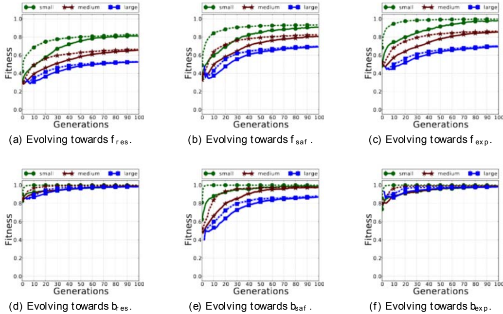
Fig. 7.1: Evolving towards a single objective for strategy game levels. Values are averaged across 50 runs. The dotted line displays the population’s maximum fitness and the solid line the population’s average fitness.
