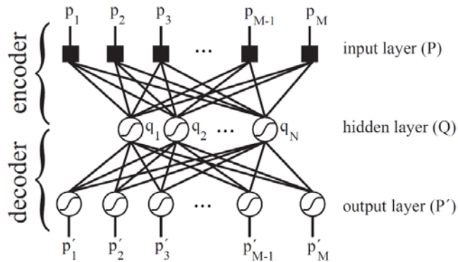
Fig. 3.1: The autoencoder architecture, consisting of the encoder where \mathbf{Q} = \mathbf{f}^w(\mathbf{P}) and the decoder where \mathbf{P}^0 = \mathbf{g}^w(\mathbf{Q}) . The higher-level representation in \mathbf{q}_1; \mathbf{q}_2; \dots; \mathbf{q}_N contains compressed information which exploits typical patterns in the training set.
