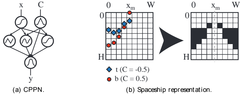
Fig. 10.12: Fig 10.12a shows a sample CPPN using the full range of pattern-producing activation functions available. Fig. 10.12b shows the process of spaceship generation: the coordinates 0 to x_m , normalized as 0 to 1 (respectively) are used as input \mathbf{x} of the CPPN. Two \mathbf{C} values are used for each \mathbf{x} , resulting in two points, top ( \mathbf{t} ) and bottom ( \mathbf{b} ) for each \mathbf{x} . CPPN input \mathbf{x} and output \mathbf{y} are treated as the coordinates of \mathbf{t} and \mathbf{b} ; if \mathbf{t} has a higher \mathbf{y} value than that of \mathbf{b} then the column is empty, else the hull extends between \mathbf{t} and \mathbf{b} . The generated hull is reflected vertically along x_m .
