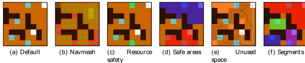
Fig. 5.5: Different map displays on a small two-player map sketch describing a strategy game level: Default displays passable tiles (light brown), impassable tiles (dark brown), resources (cyan) and player bases (white). Navmesh displays the passable pathways on the map and the location of choke points (red), dead ends (black) and open areas (yellow); Resource safety displays the safety value of each resource (in shades of green) and connects bases to their safe resources. Safe areas shows the tiles close to each base (here in red and blue) which are considered safe. Unused space shows all shortest paths between bases and resources, and highlights leftover unused space (orange). Segments shows the passable areas (in different colors) which are surrounded solely by chokepoints.
