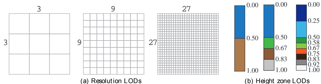
Fig. 10.3: The Levels of Detail (LOD) used for the map sketches in Sentient World (from left to right: LOD of 1, 2 and 3), in terms of grid resolution and height zones. Numbers in Fig. 10.3a refer to the number of tiles available in each row and column for that LOD, while numbers in Fig. 10.3b refer to the lower and upper bounds ( l_i; u_i ) of each corresponding height zone.
