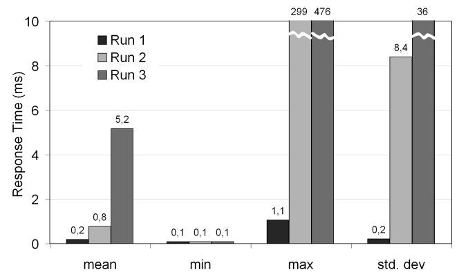
Figure 5: The graph shows the mean, min and max response time for the sequential writes on P2 for each run. The Intel X25-M is not bimodal because the cost of sequential writes is not constant across runs.
