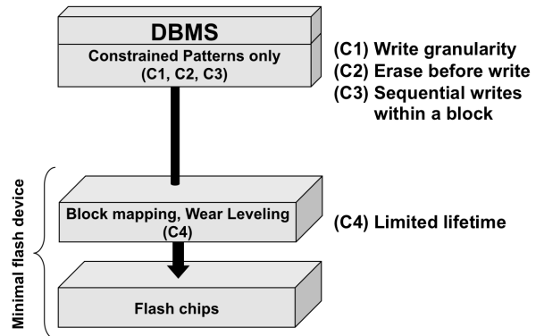
Figure 1: Minimal FTL does not support updates or random writes but offers optimal performance for IO patterns respecting C1, C2 and C3.
