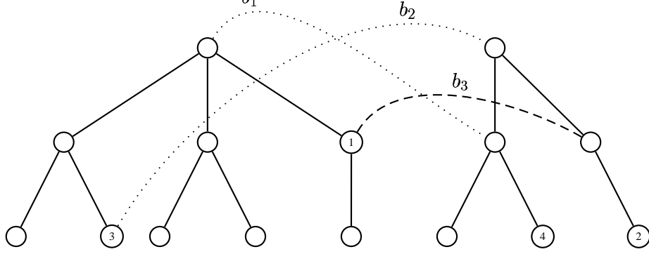
Figure 1: The solid lines are tree edges and the dashed and dotted lines are bridges of color c and c' , respectively. \text{firstcolorbridge}(c, v_1, v_2) returns b_3 . \text{firstcolorbridge}(c', v_3, v_4) returns ambiguity since neither b_1 or b_2 is closer than the other.
